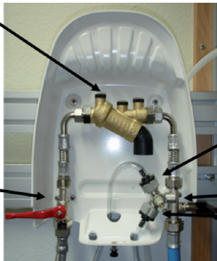
Honeywell Systemtrenner
